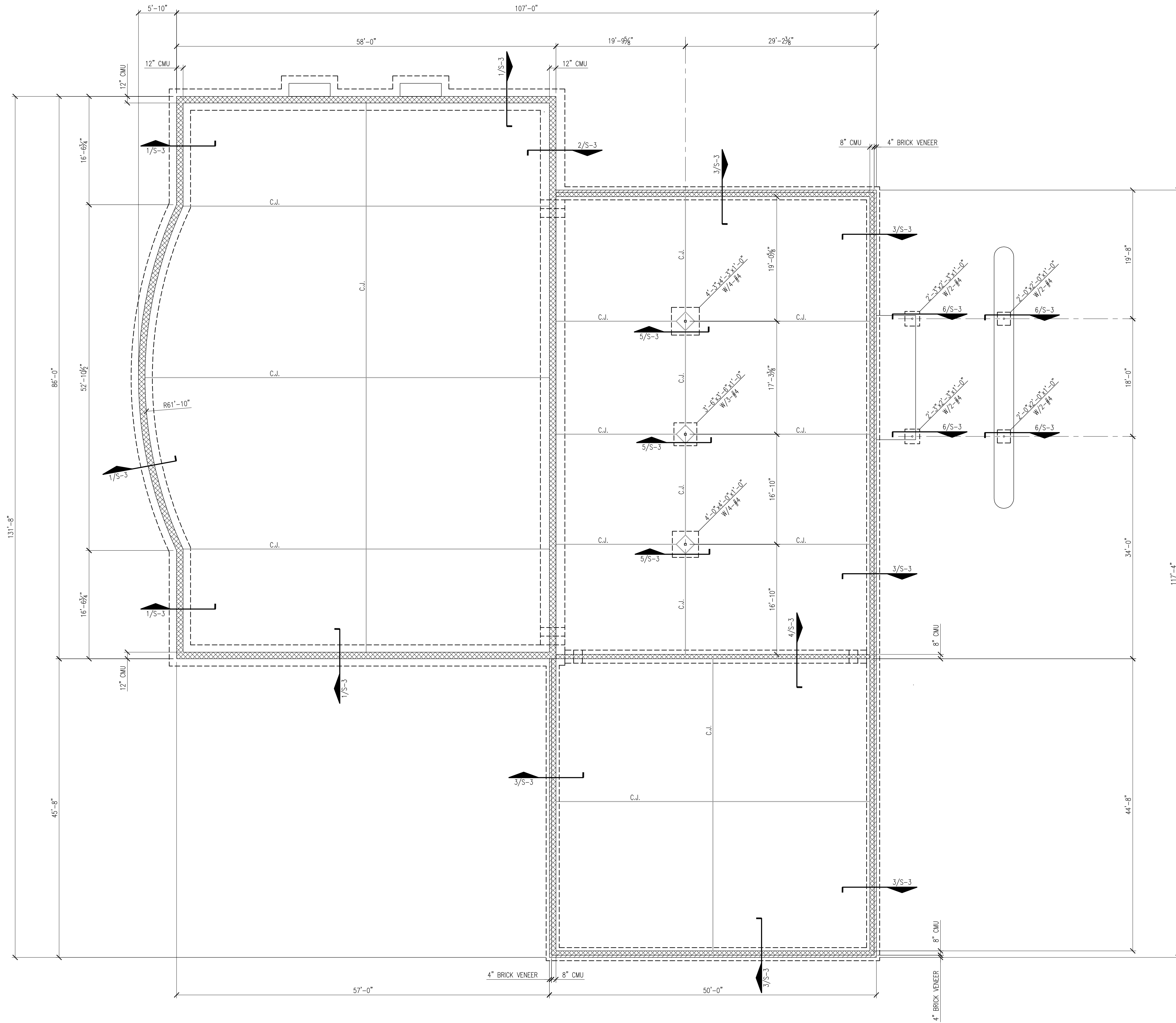
1 FOUNDATION/FIRST FLOOR PLAN S-1 SCALE: 1/8"=1'-0"
