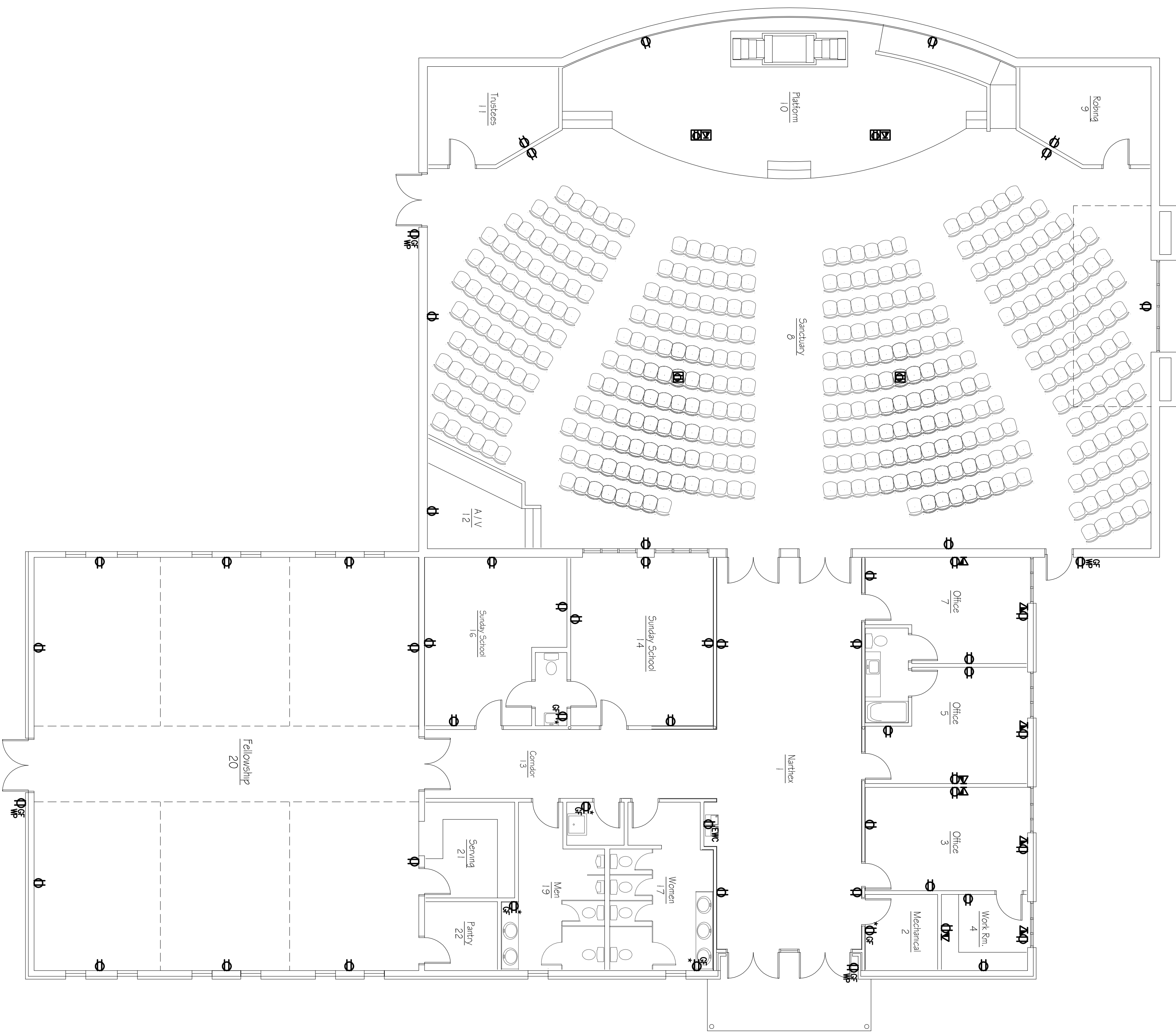
1 Floor Plan - Electrical E-2.0/1/8 - 1-D
