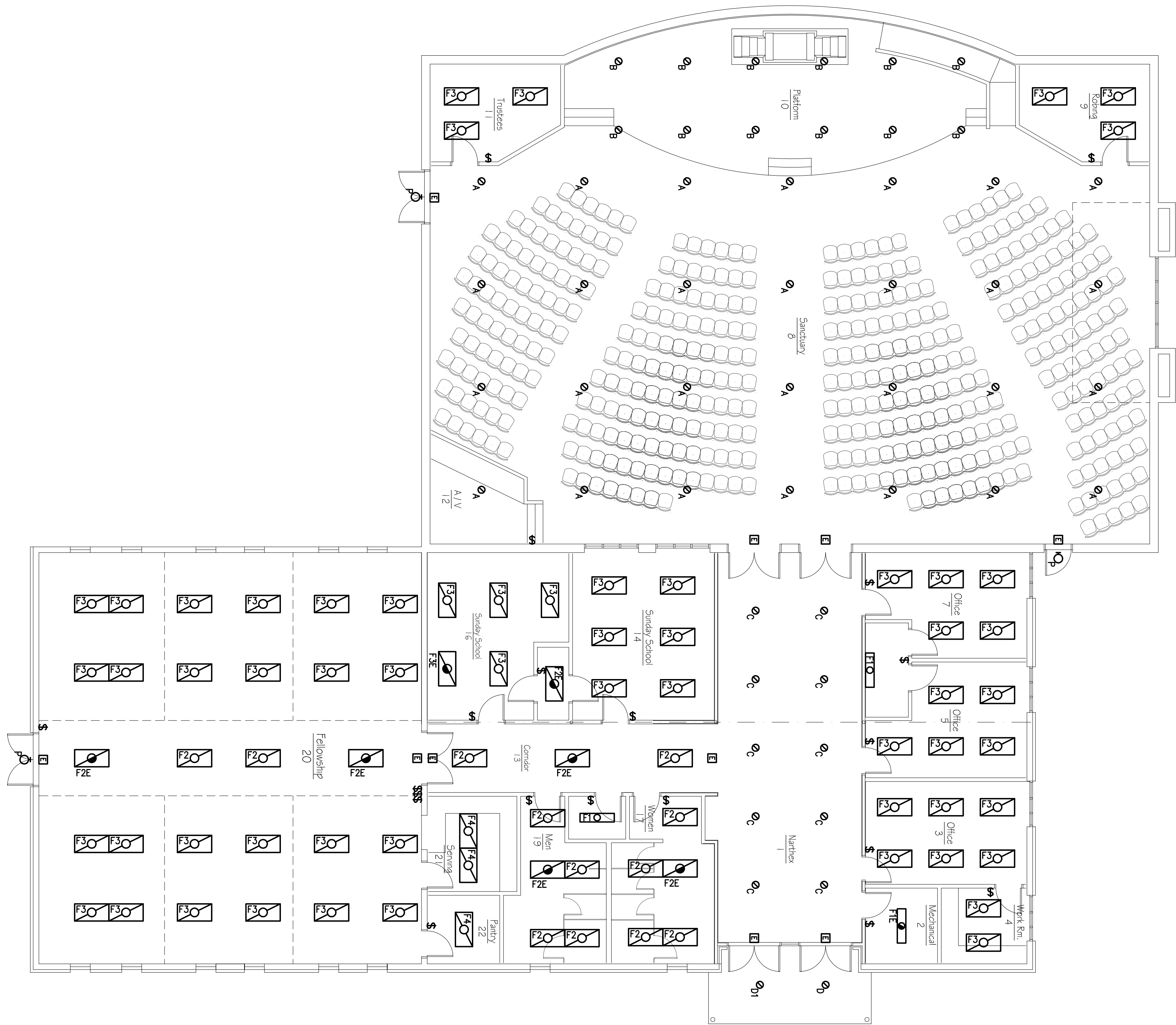
1 Ceiling Plan - Electrical E-3.0 / 1/8" = 1'-0"
