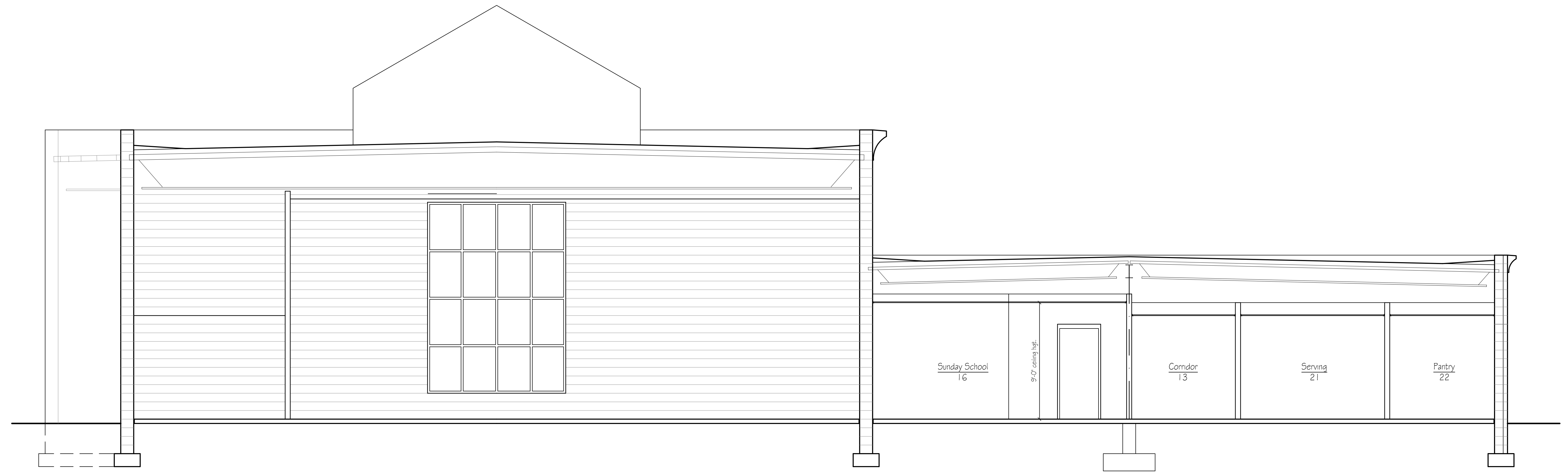
2 Building Section A-4 1/4" = 1'-0"
